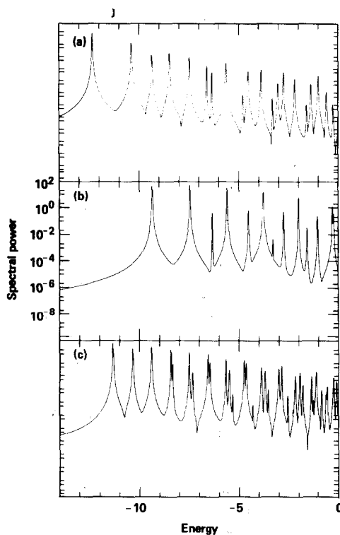
FIG. 6. Energy spectra for Hénon-Heiles potential below the dissociation energy for states of three main symmetries (a) R = 1, \sigma_r = 1 ; (b) R = 1, \sigma_r = -1 ; (c) R = \exp(i2\pi/3), \exp(-i2\pi/3) (degenerate states).
